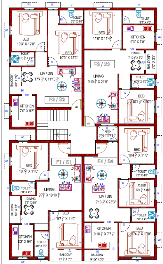
FIRST / SECOND FLOOR PLAN
